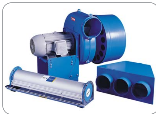
Several sizes of direct or self-tensioning belt drive blowers available.
